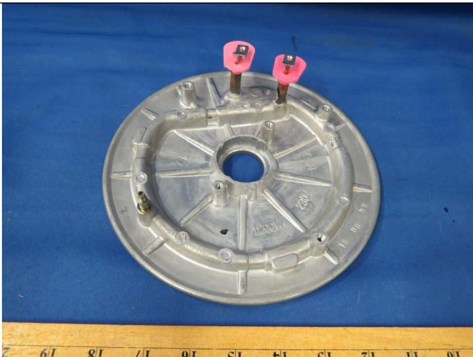
Bottom Heater View
