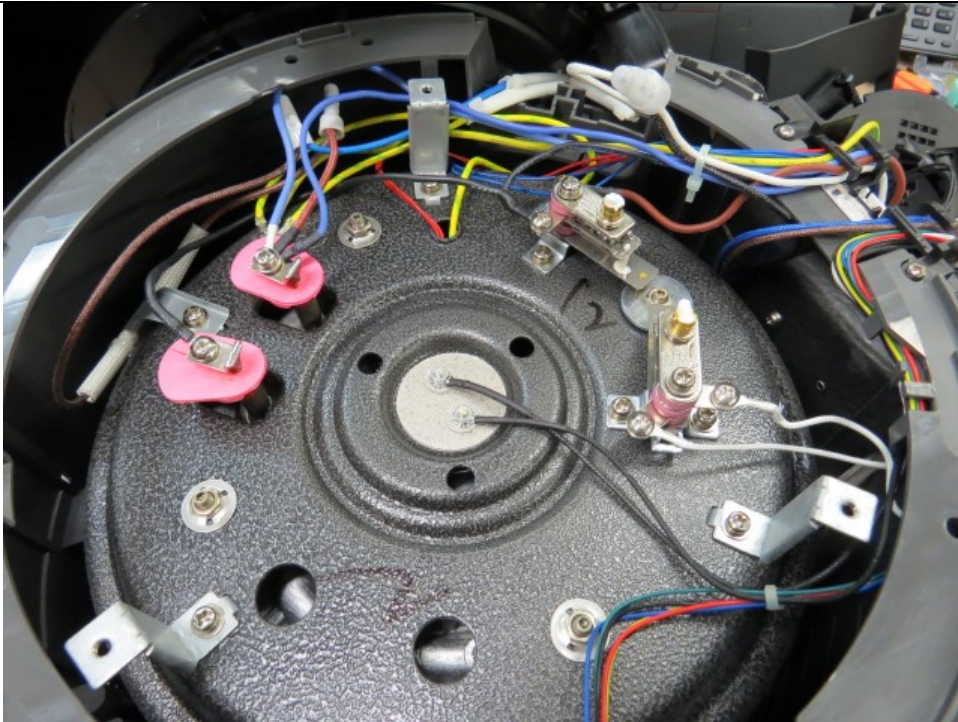
Internal View of Main Unit
