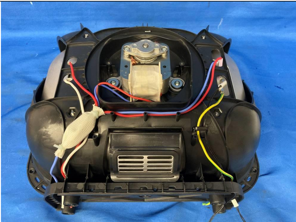
Internal View of AF Lid
