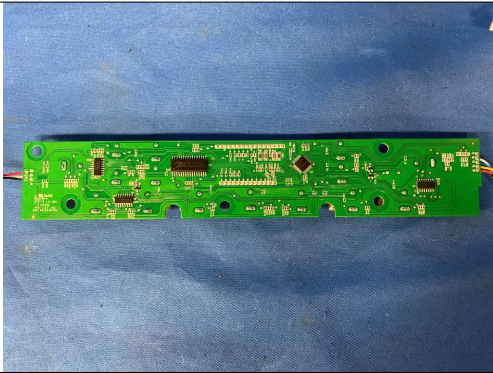
UI PCBA, track side
