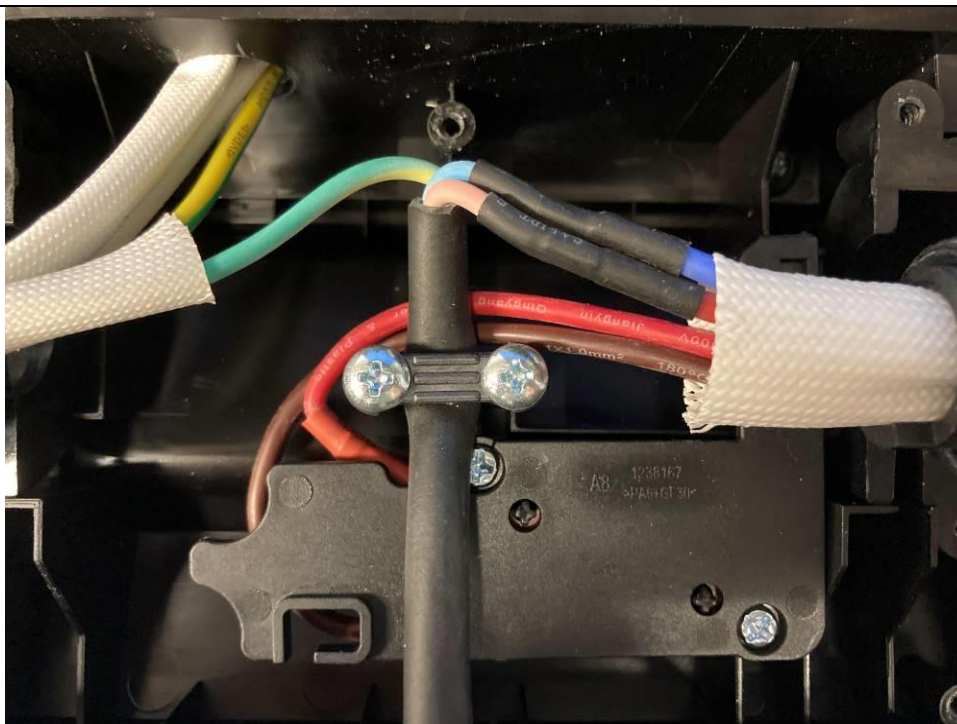
Cord Anchorage View
