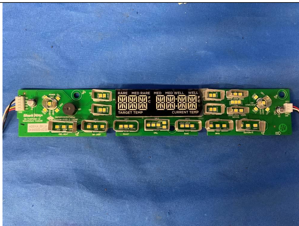
UI PCBA, component side
