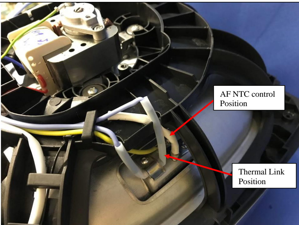
View of thermal link and AF NTC control
