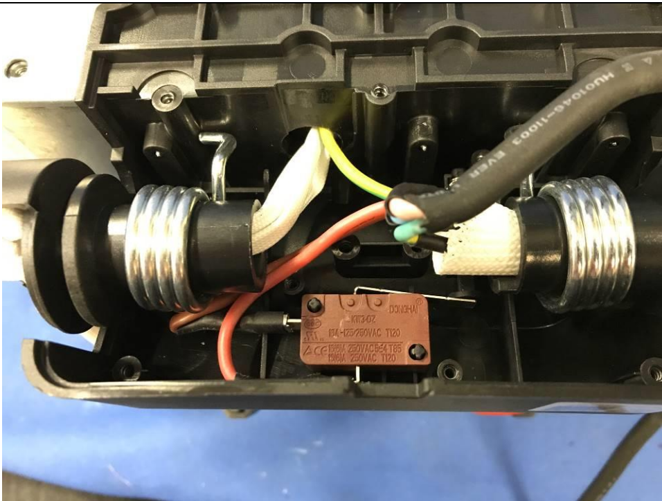
Interlock Switch View
