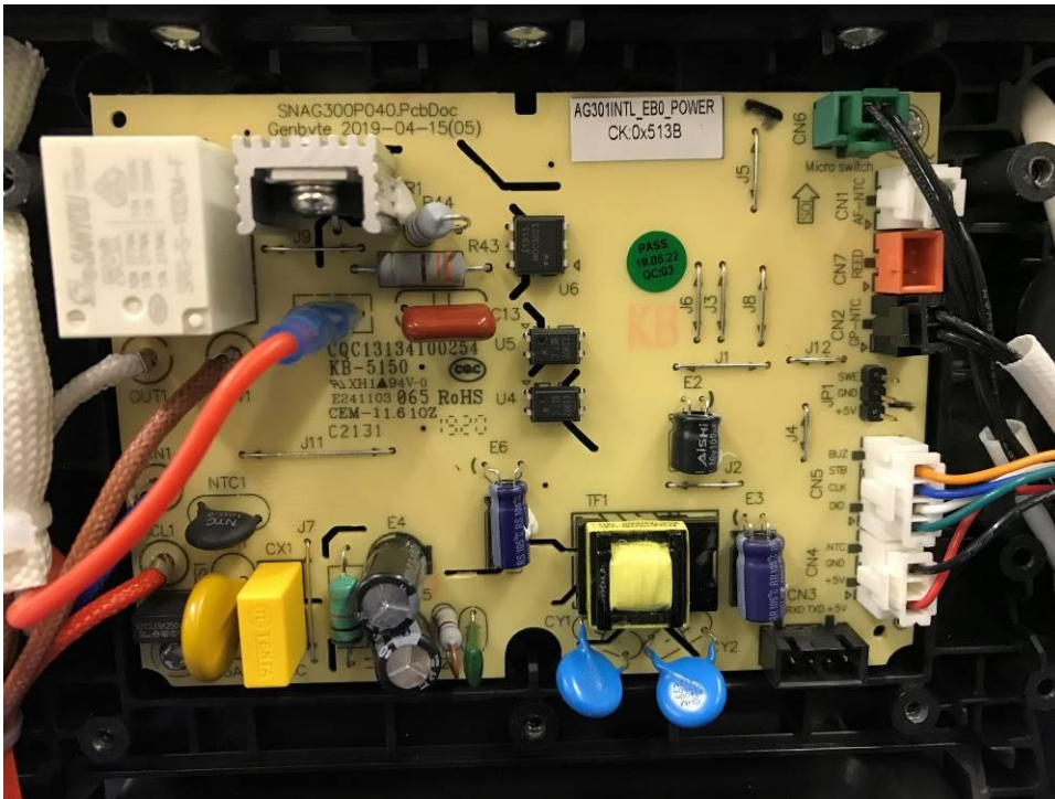
Power PCBA, component side
